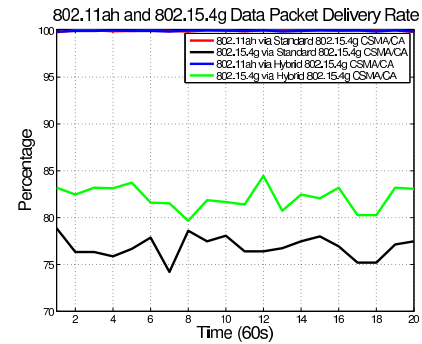
Figure 15: Scenario-5: Packet Delivery Rate
