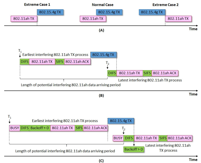
Figure 4: 802.11ah TX interfering with 802.15.4g TX
