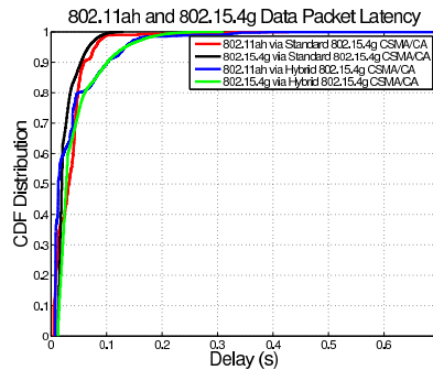
Figure 10: Scenario-2: Packet Latency
