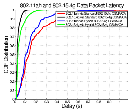
Figure 14: Scenario-4: Packet Latency
