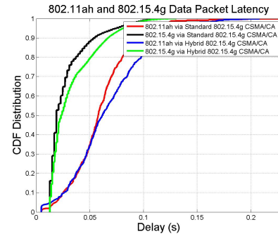
Figure 12: Scenario-3: Packet Latency
