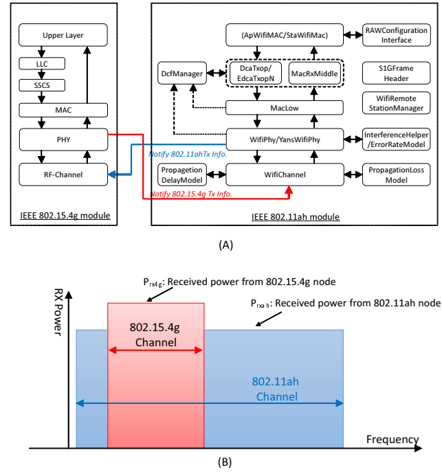
Figure 5: Sub-1 GHz Band Coexistence Simulator Model Interface
