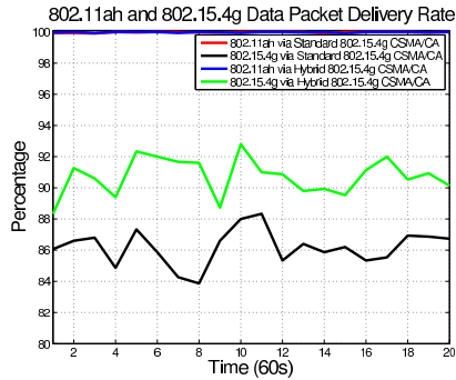
Figure 9: Scenario-2: Packet Delivery Rate
