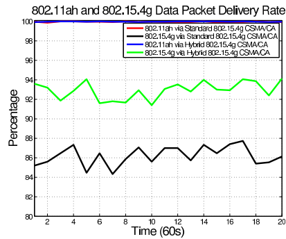
Figure 13: Scenario-4: Packet Delivery Rate
