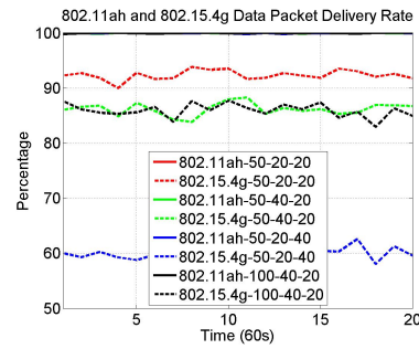
Figure 1: Packet Delivery Rate
