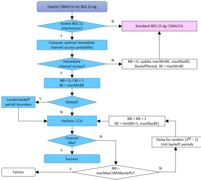
Figure 3: Hybrid CSMA/CA for IEEE 802.15.4g
