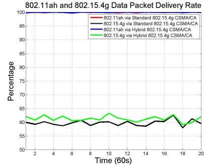
Figure 11: Scenario-3: Packet Delivery Rate
