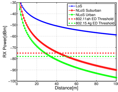
Figure 6: ITU-R P.1411-9 Propagation Model
