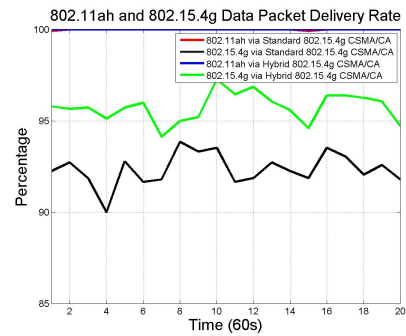
Figure 7: Scenario-1: Packet Delivery Rate
