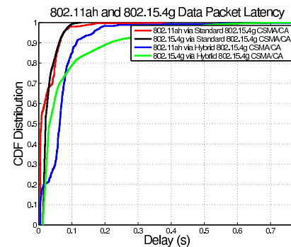
Figure 16: Scenario-5: Packet Latency
