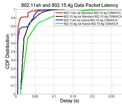
Figure 8: Scenario-1: Packet Latency
