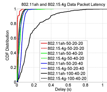
Figure 2: Packet Latency
